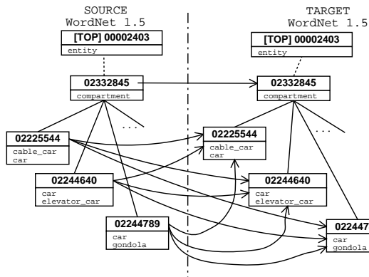
Figure 6: Example of ambiguity in leaf nodes
